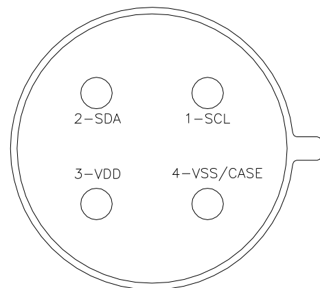
Figure 4. Package Top View
